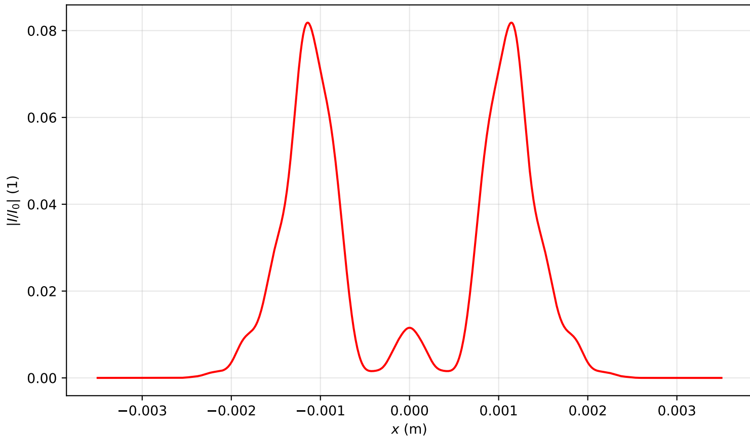
Intensity profile I(x, y = 0, z = 3.344)/I_0 , P_{in}=7.5P_{cr} , artificial time
